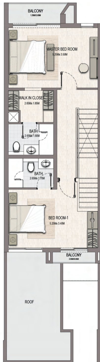
First Floor
