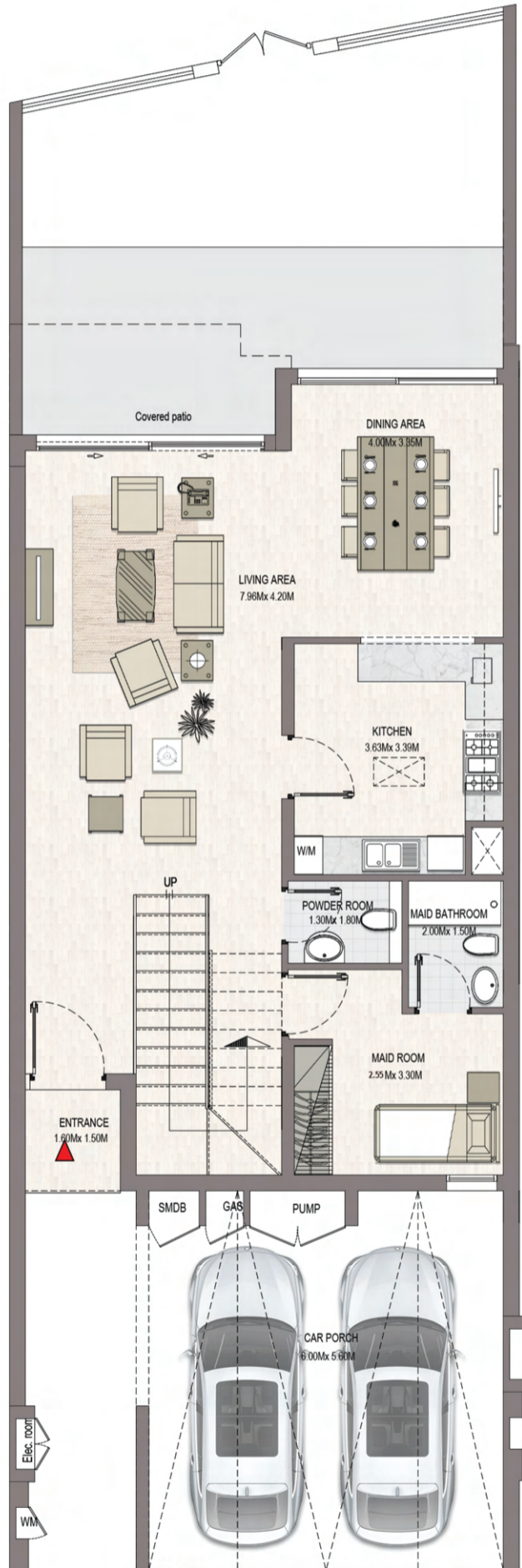
Ground Floor
