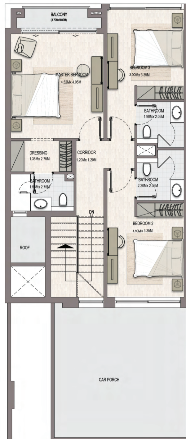
First Floor
