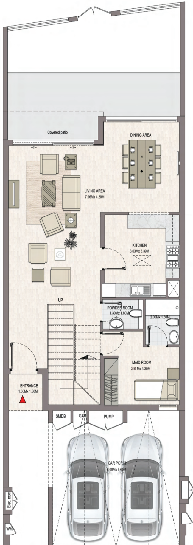
Ground Floor
